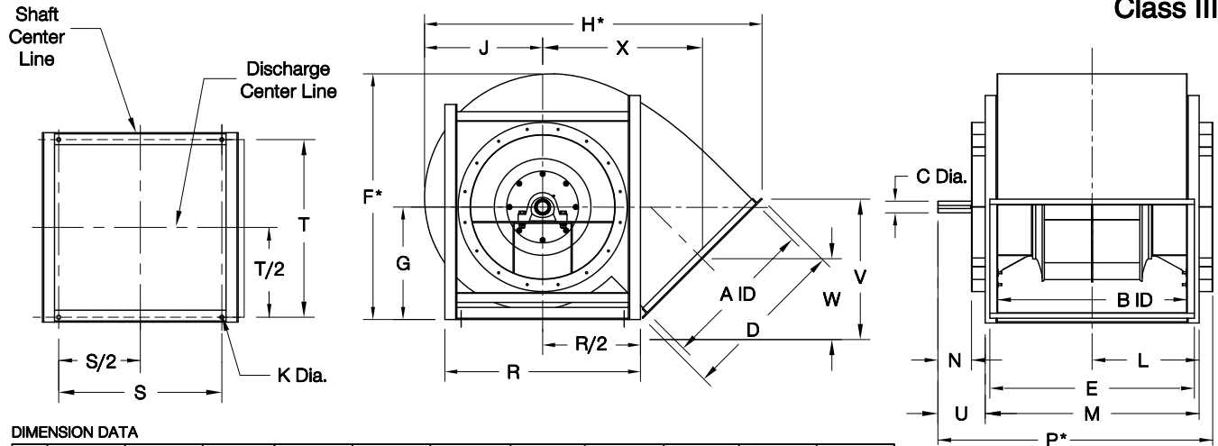
DIMENSION DATA
