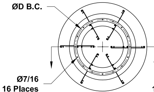
CAVP / Remote Mount Nozzle
