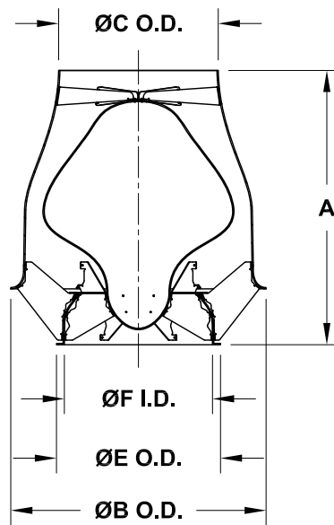
CAVP / Remote Mount Nozzle
