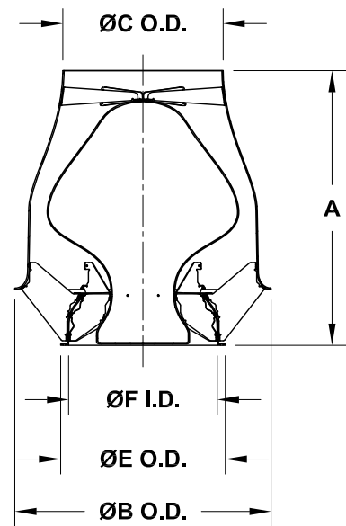
QMX Nozzle
